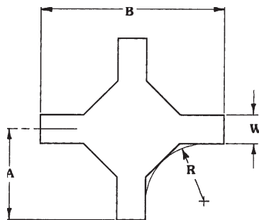
Cross
